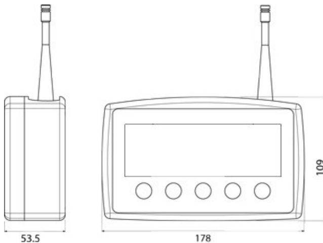
DFWPM: dimensions in mm.
