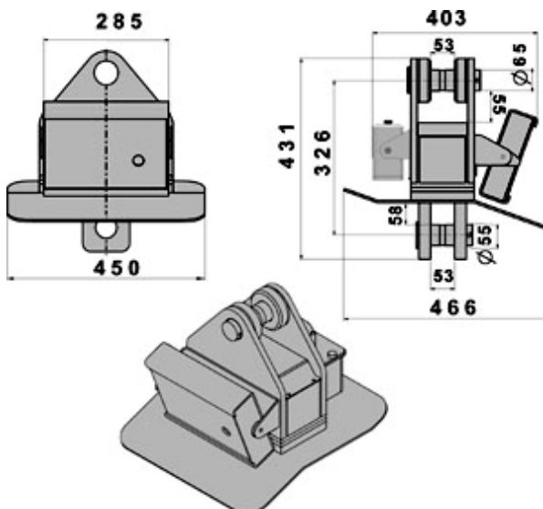
MCWATEX - dimensions in mm
