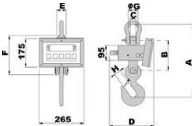
MCW dimensions (capacities 150 - 6500 kg)
