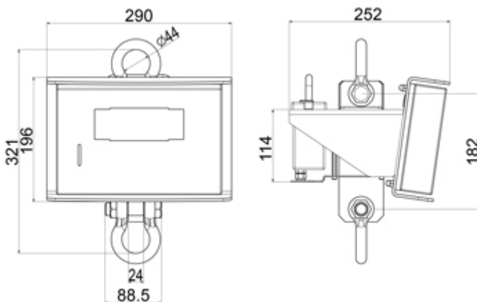
MCWX2GD - dimensions in mm.
