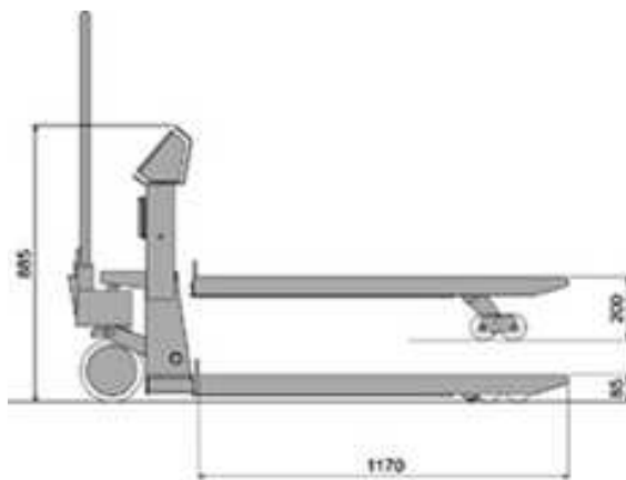
TPWX3GDI: pallet truck scale in STAINLESS steel, for hazardous zones.
